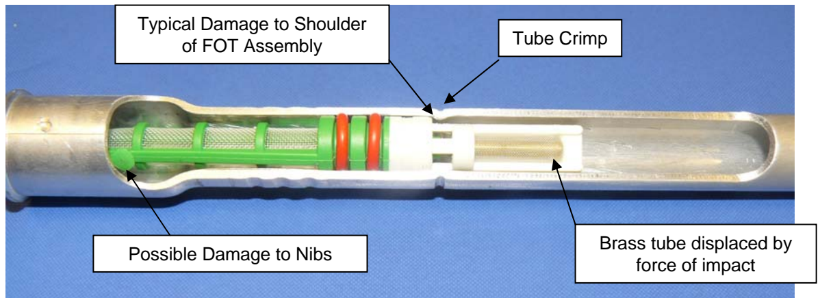
Figure 3: FOT Assembly moves rapidly into the tube crimp during the evacuation and fill process or during high compressor loads and pressure. The brass tube will continue to move out of position. A/C system may not function properly due to flow restrictions.
