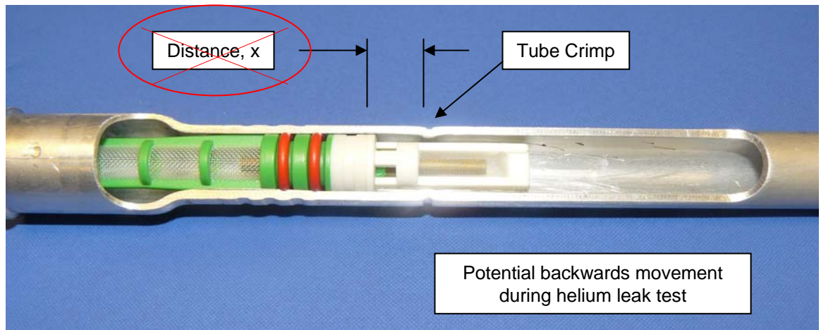
Figure 2: IMPROPERLY seated FOT Assembly against the Aluminum tube crimp.
