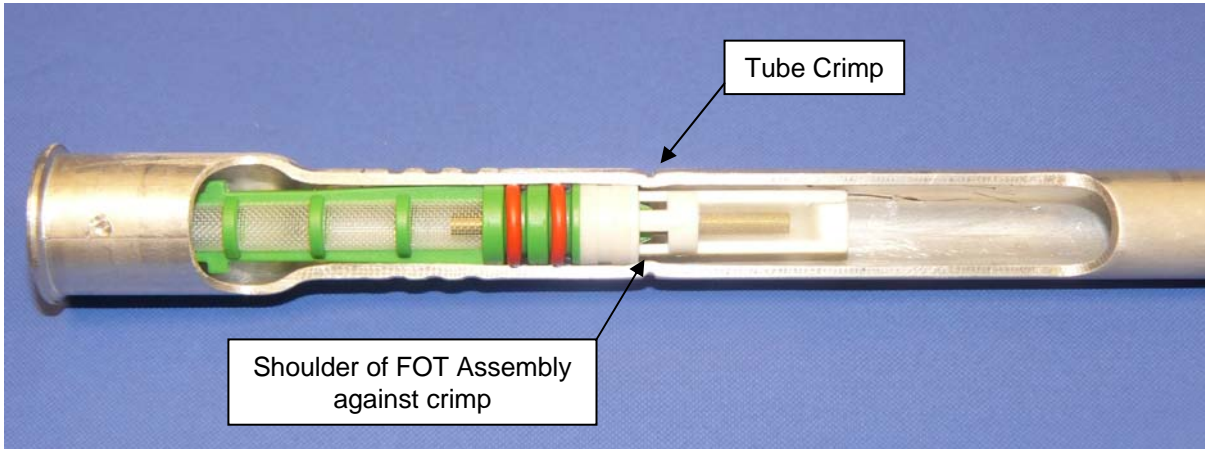
Figure 1: PROPERLY seated FOT Assembly against the Aluminum tube crimp.
